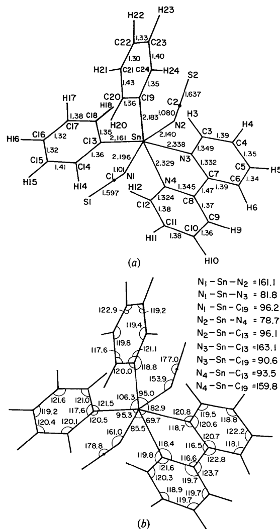
Fig. 2. (a) Atom names and bond distances (Å) (uncorrected for thermal motion). The e.s.d.'s on bond distances involving Sn are \sim 0.005 Å, involving H are \sim 0.07 Å and for the other atoms range from 0.005–0.01 Å. (b) Angles (°) in the molecule. The e.s.d.'s on angles involving Sn are \sim 0.2^\circ and for the others \sim 0.8^\circ .
